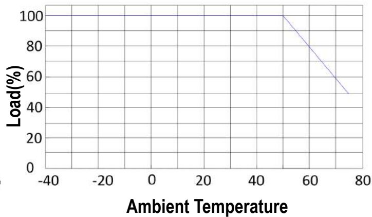
Output Load VS Temperature
