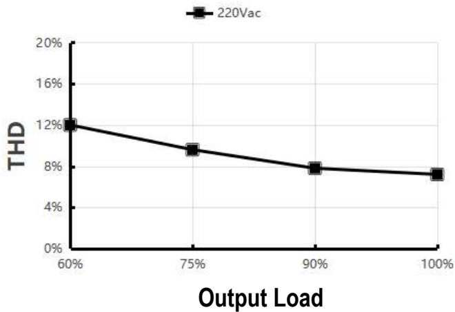
THD Vs Output Load
